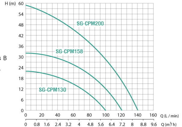
Performance curve
