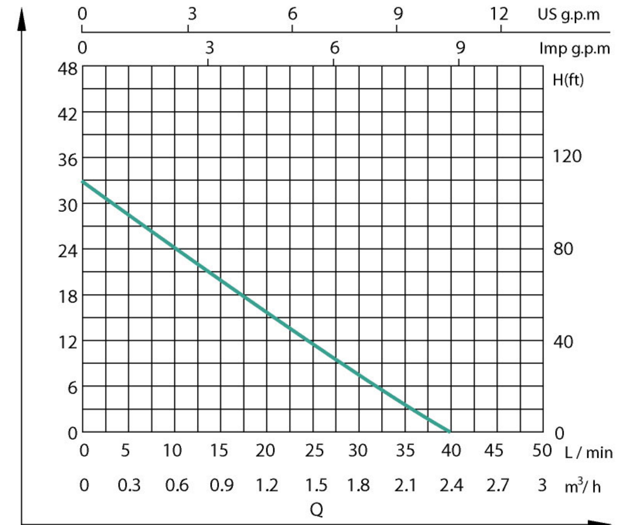
Performance curve
