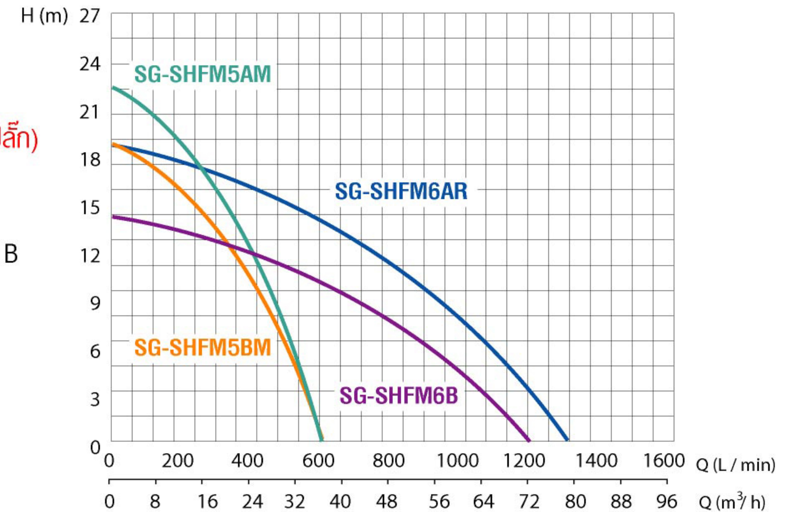
Performance curve
